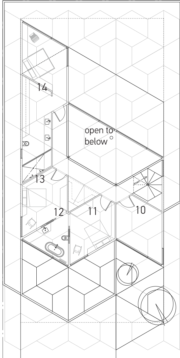
SECOND FLOOR.
