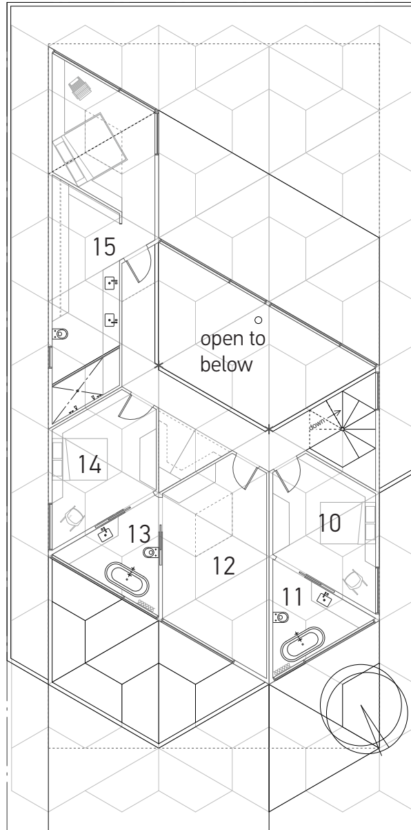
SECOND FLOOR.
